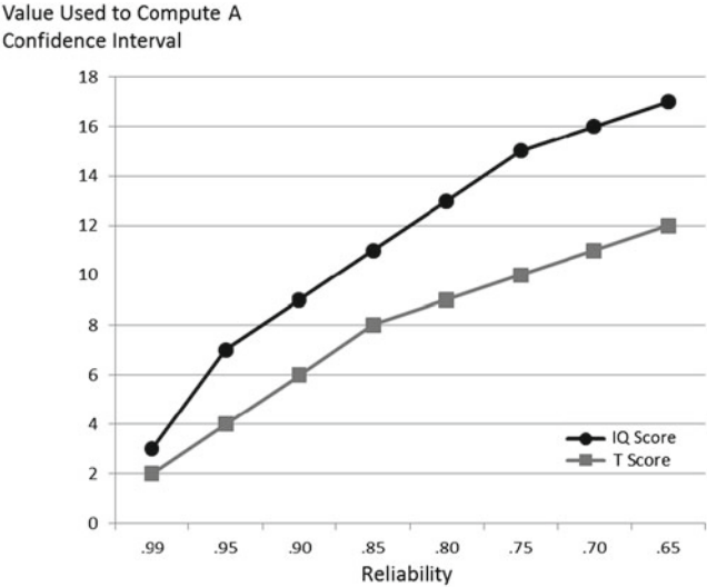
Fig. 14.1 Relationship between reliability and confidence intervals
